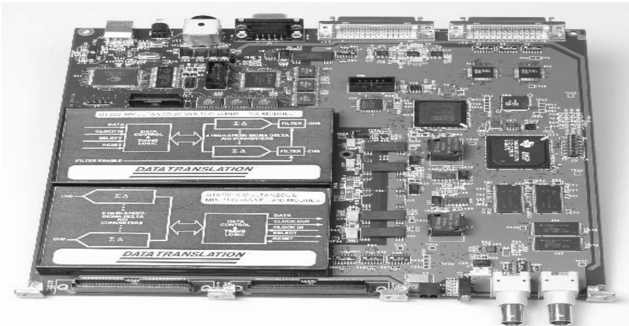
FIG. 2 – DT9841 FULCRUM II SERIES WITH TI C6711 FLOATING-POINT DSP
