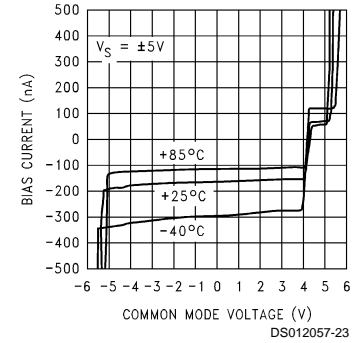
Bias Current vs V_{CM}
