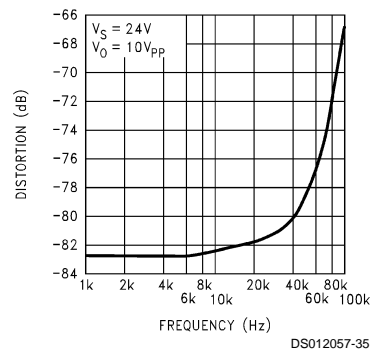
Distortion + Noise vs Frequency
