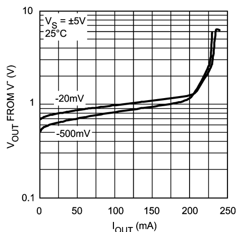
FIGURE 5. I_{SINK} vs. V_{OUT} (for Various Overdrive)
